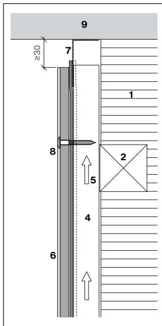
Detalj under platta
