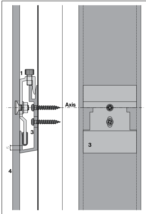
U-cleat and hook-in cleat with adjustment
