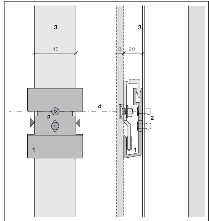
Attachment: 2 rivets per U-cleat, 4.8 \times 12 -K9.0 mm Remove drill chips from the U-cleats
