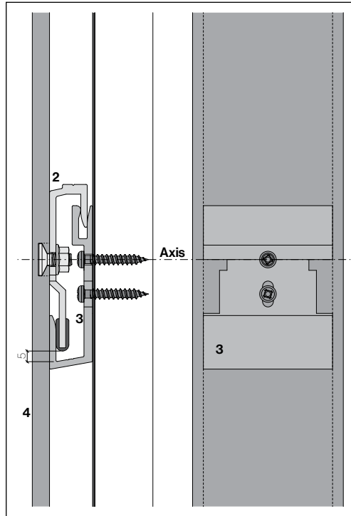
U-cleat and hook-in cleat
