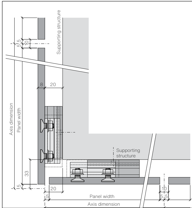
Planning aid, dimensioning of the axes at the outer corners
