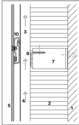
Wood/metal sub-construction heat bridge optimized sub-construction
