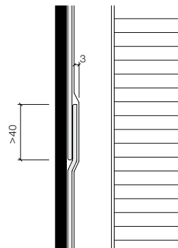
Overlappend EPDM-voegband
