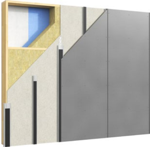
Light wall with vertical VFL steel profiles
