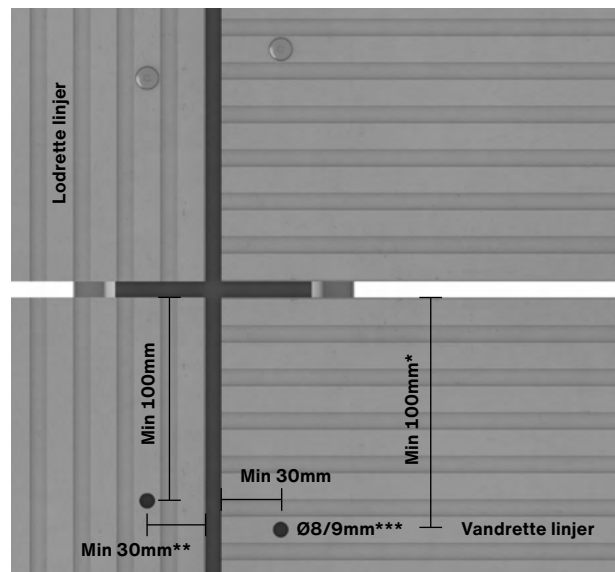
Fig. 3. Swisspearl Patina Inline edge distances. Note! Min distance and/or the nearest following top line. ***9mm drill bit for rivet and a 8mm drill bit for screws.
