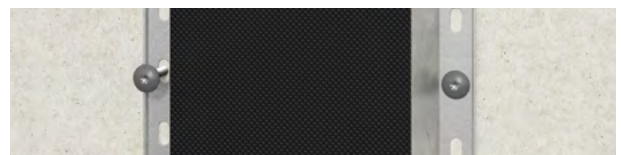
Fig.2. Sliding points: Swisspearl VFL profiles are installed with fastener in the center of the elongated holes
