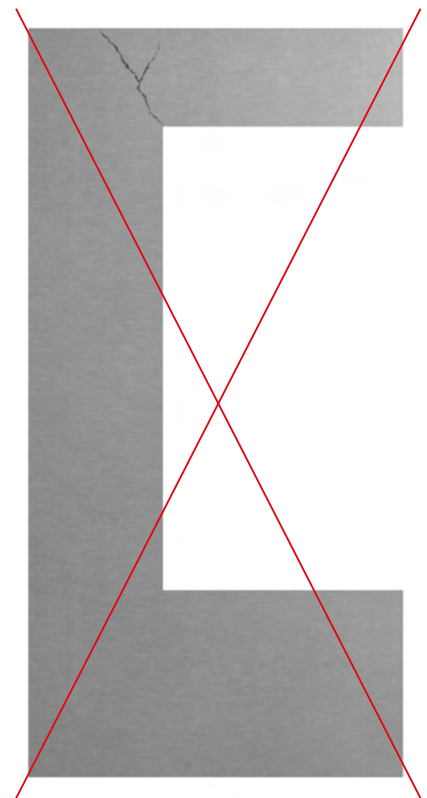
Fig. 3. Incorrect installation of Swisspearl facade boards at windows, doors and openings.
