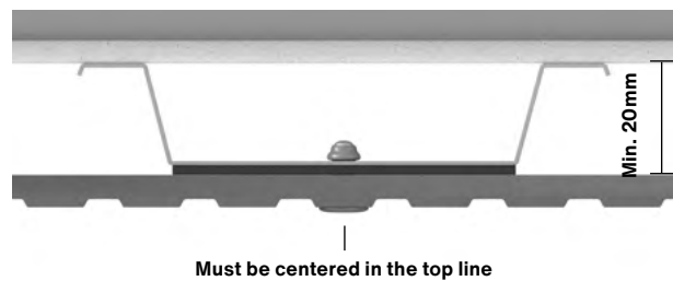
Fig. 2. Swisspearl Patina Inline installation on the middle profile.
