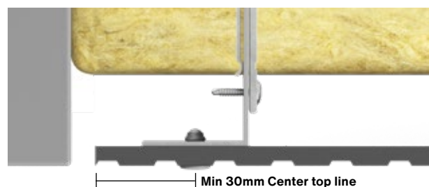
Fig. 4. Swisspearl Patina Inline installation on cut to size board.
