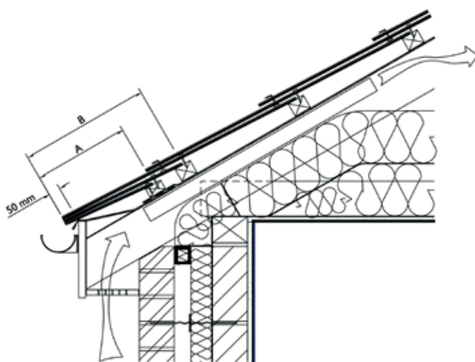
Standard eaves with soffit ventilation.
