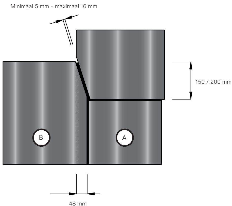
Fig 5.0 – Verticale overlap
