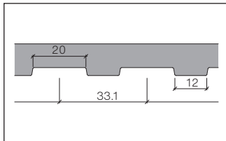
Detail Gravurraster Gravail
