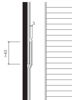
EPDM strip overlap
