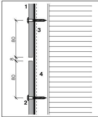
Offene Horizontalfuge
