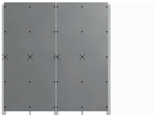
Example: Vertically mounted boards with one intermediate aluminium profile
