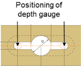
Check of borehole geometry: depth of borehole
