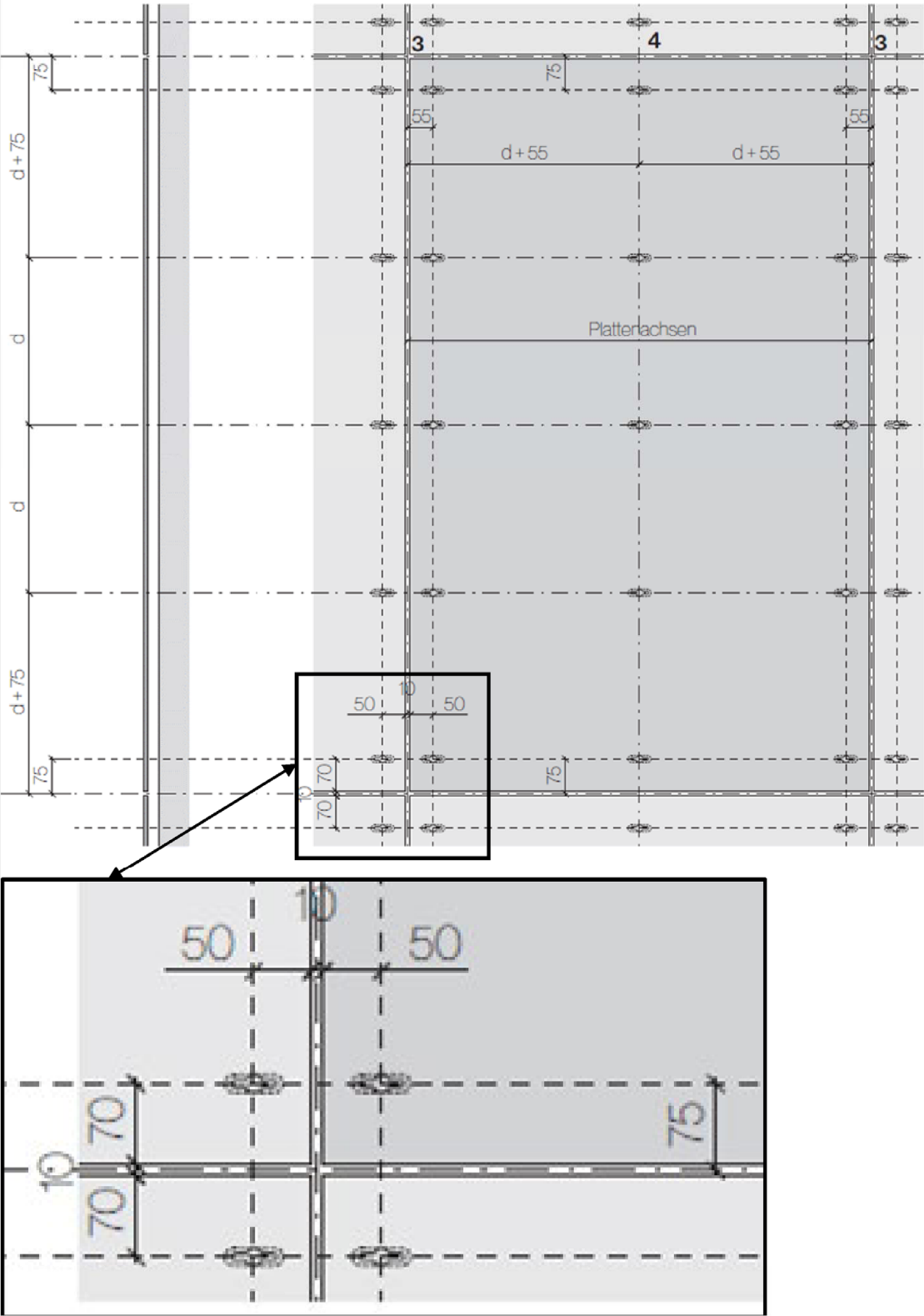
Edge distances and distances between anchors:
