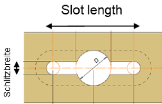
Check of borehole geometry: Length of undercut
