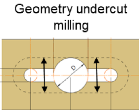
Check of borehole geometry: diameter of plunge milling
