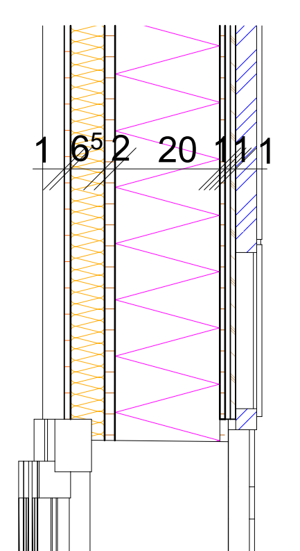
Detail AW 01 M 1:10
