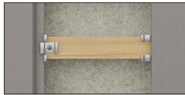
Picture 2 Swisspearl Connect clip
