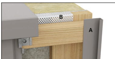
Picture 7 A. Swisspearl Plank Connect End Profile B. Swisspearl Ventilated Profile
