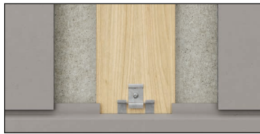
Picture 2 Swisspearl Plank Connect Clips
