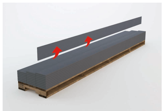
Do not drag products from the pallet, as it may leave permanent scratch marks. Lift the product by its narrow edge as it may break if handled incorrectly.
