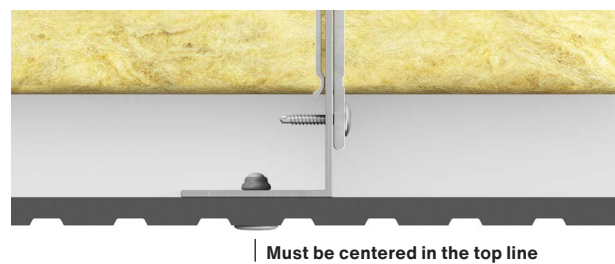
Fig. 2. Swisspearl Patina Inline NXT installation on L profile.
