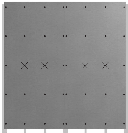
Example: Vertically mounted boards with two intermediate aluminum profile
