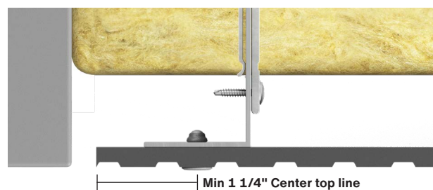
Fig. 4. Swisspearl Patina Inline NXT installation on cut to size board.
