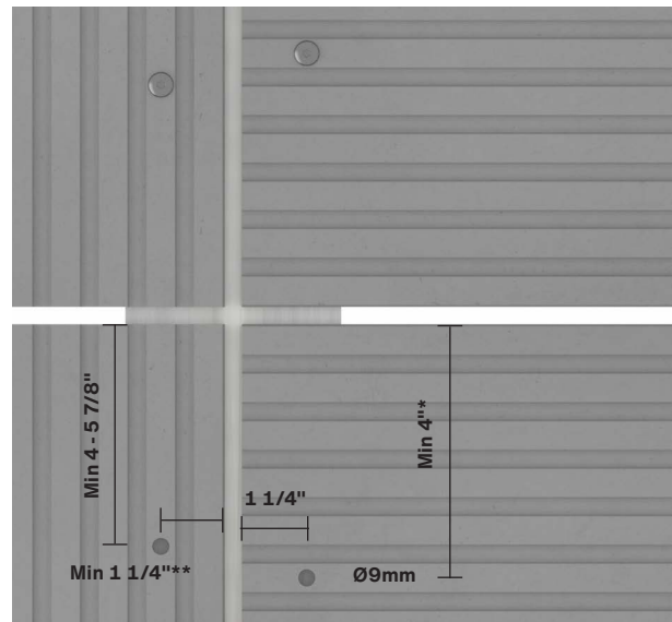
Fig. 3. Swisspearl Patina Inline NXT edge distances. Note! Min distance and/or the nearest following top line.
