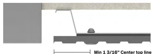
Fig. 4. Swisspearl Patina Inline installation on cut to size board.
