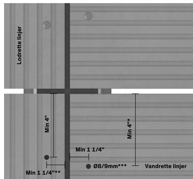
Fig. 3. Swisspearl Patina Inline edge distances. Note! Min distance and/or the nearest following top line. ***9mm drill bit for rivet.
