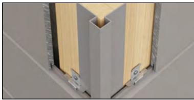
Picture 1 Swisspearl Plank Connect External Corner Profile Small
