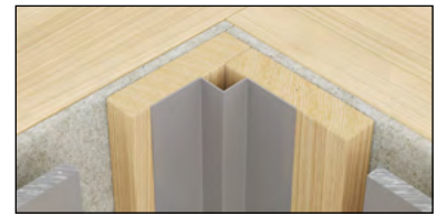
Picture 3 Swisspearl Plank Connect Internal Corner Profile
