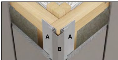
Picture 1 A. Swisspearl Plank Connect Startprofile B. Swisspearl Plank External Corner Small
