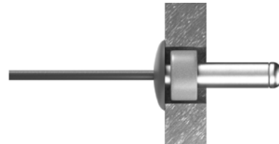
X : Fixing position hole diameter \varnothing 9 mm. Insert a Swisspearl Fixing Sleeve in the hole before the rivet is fixed.
