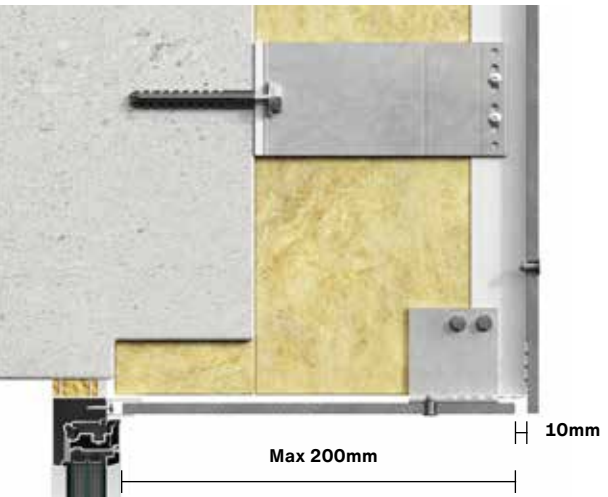
Vertical view: Window head As with jambs, the window head can be formed using Swisspearl boards. At the front edge of the head detail, ensure a minimum free opening area of 10mm, or equivalent 100cm 2 per meter to ensure adequate ventilation behind the facade. Use a Swisspearl Ventilated Profile to ensure that insects and vermin cannot enter the construction behind the facade board.
