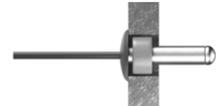
X : Fixing position hole diameter Ø9 mm. Insert a Swisspearl Fixing Sleeve in the hole before the rivet is fixed.
