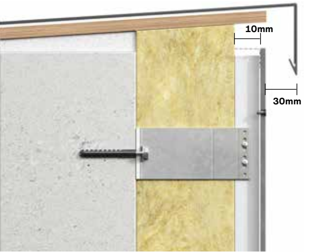
Vertical view: Top construction Make sure that air can move freely from throughout the construction. There should be a minimum free open area of 10mm, or equivalent 100cm 2 per meter to provide adequate ventilation throughout the system. There should be a minimum gap of 30mm between the front face of the facade board and the drip edge of the capping.
