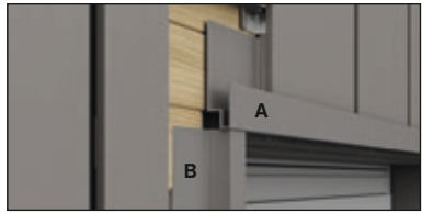
Picture 4 A. Swisspearl Plank Connect Window Profile B. Swisspearl External Corner Profile
