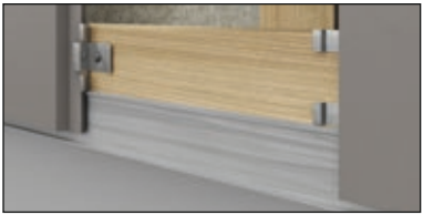
Picture 6 Swisspearl Plank Connect Vertical Start Profile
