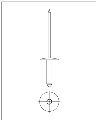
Swisspearl neet Ø 15 mm 4,0 × 18-K15
