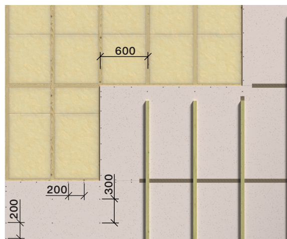
Horizontal installed Swisspearl Windstopper boards
