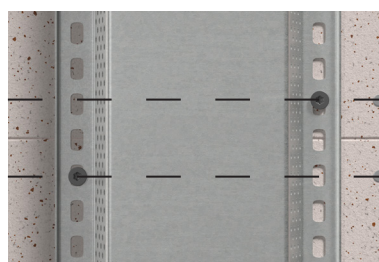
For center battens, ensure that you do not place nails too close to the edge of the underlying structure
