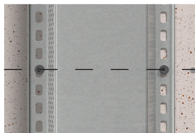
The same rules also apply to the placement of screws or bolts for securing steel profiles. Picture shows vertical installed hatprofil that are fixed into horizontally substructure behind the Swisspearl Windstopper
