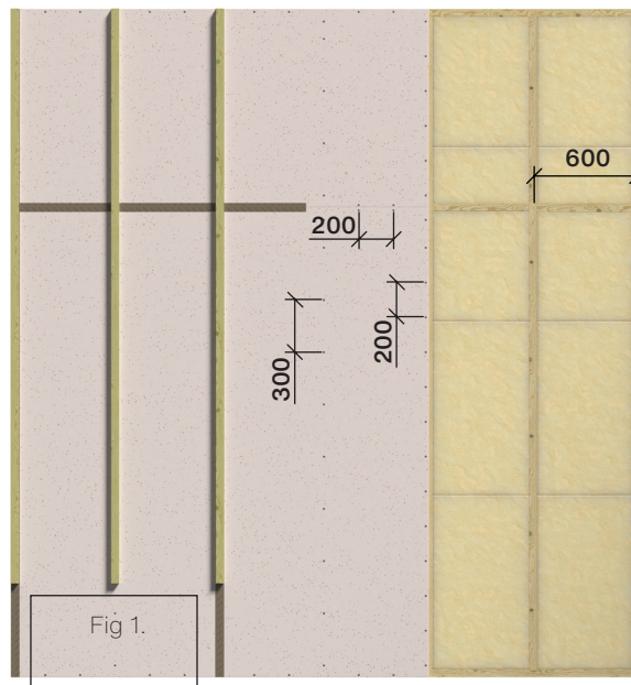
Vertically installed Swisspearl Windstopper boards
