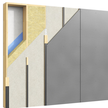
Example of a light wall structure with a A1 classified Swisspearl Windstopper Extreme 9.0 mm that also has a covering class of K 1 10 B-s1,d0, K 2 10
