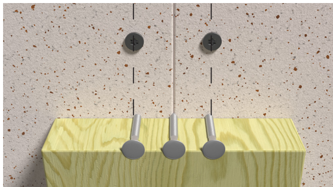
Example of nail placement in a batten beneath joints. The nail should either be positioned in the center where the panels meet or at the same spacing as the panels fixation distance
