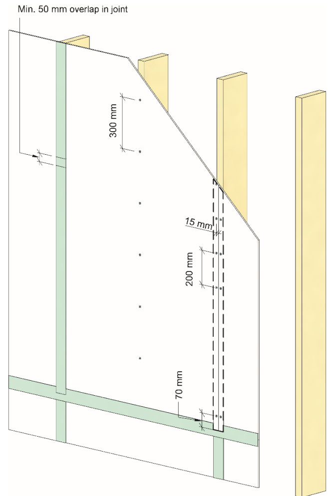
Fig. 1 Swisspearl Windstopper installed on timber studs with tape over all joints.
