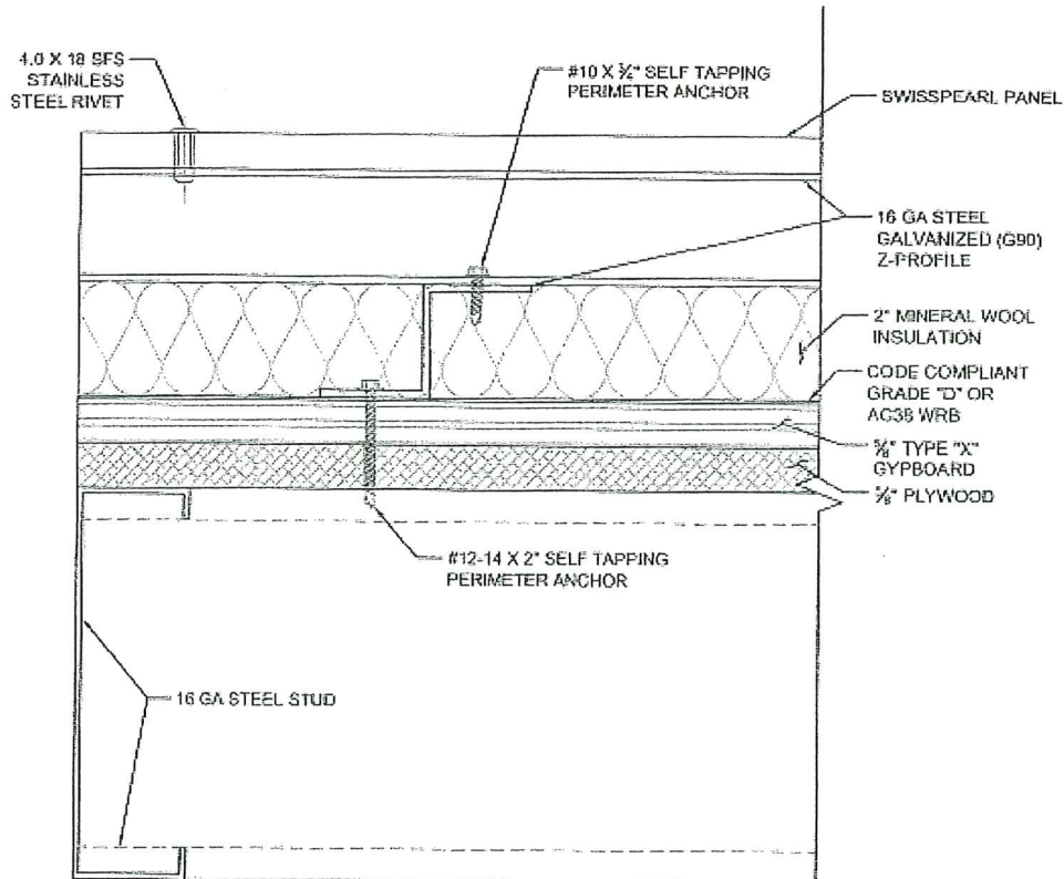
SWISSPEARL PLAN DETAIL (4' SIDE)
