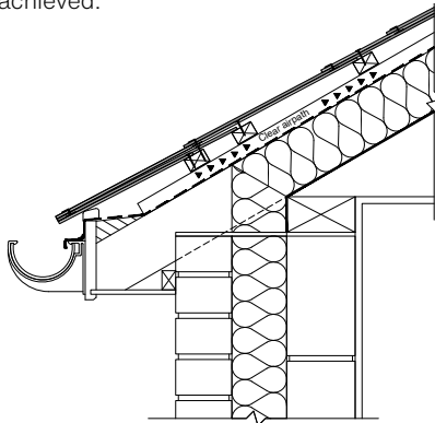
Fibre cement slate roof with LR underlay and ventilated counterbatten void.
