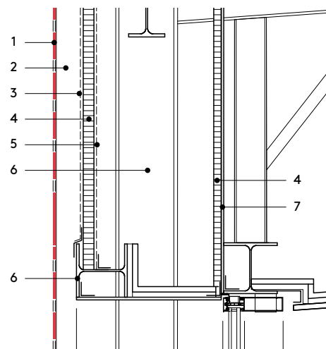
Vertical section 1:20
