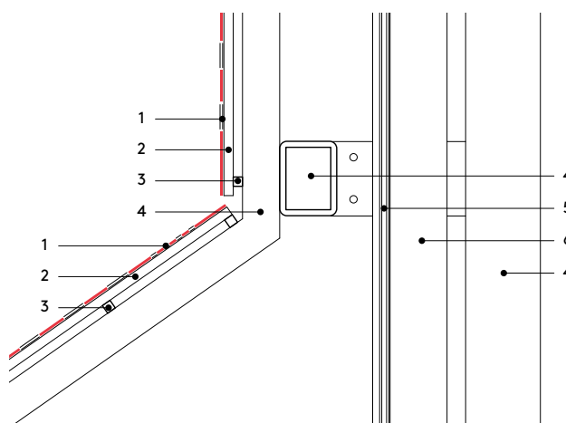
Vertical section 1:20
