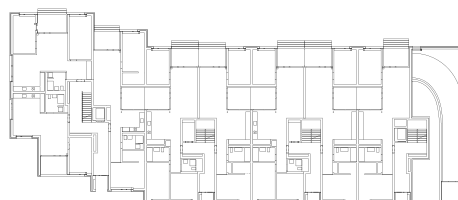
First floor 1:1000
