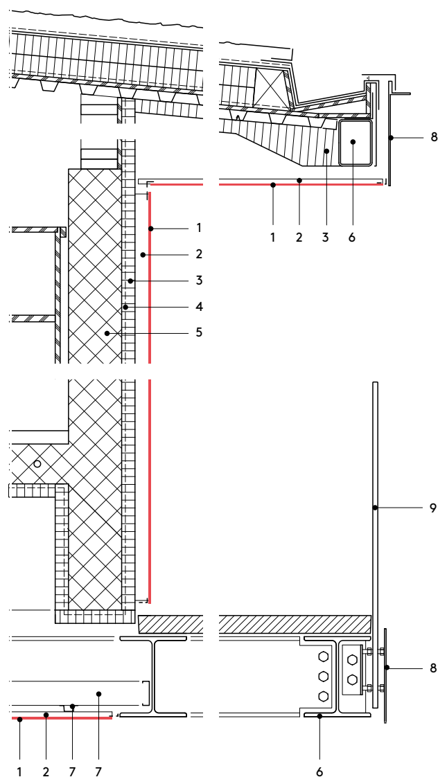
Vertical section 1:20
