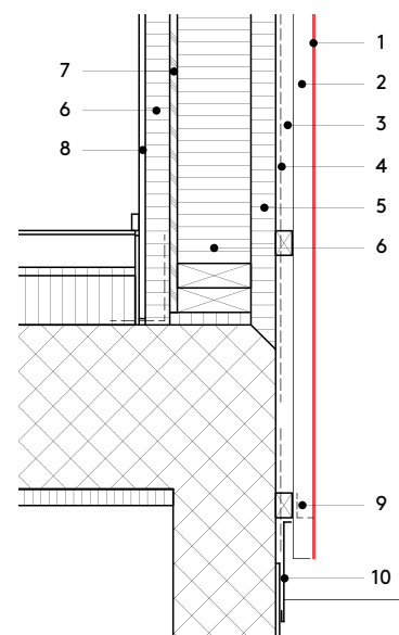
Vertical section 1:20
