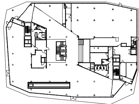
First floor 1:1000
