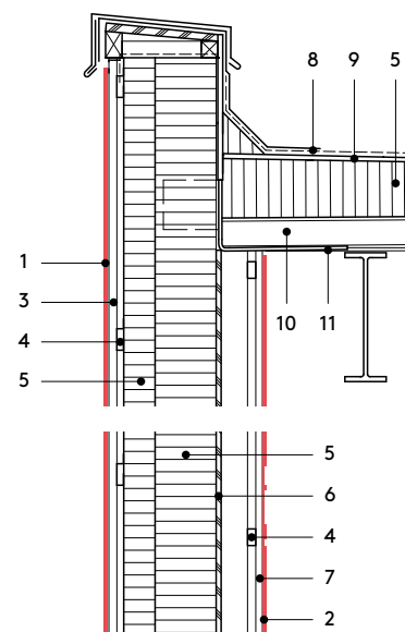
Vertical section 1:20
